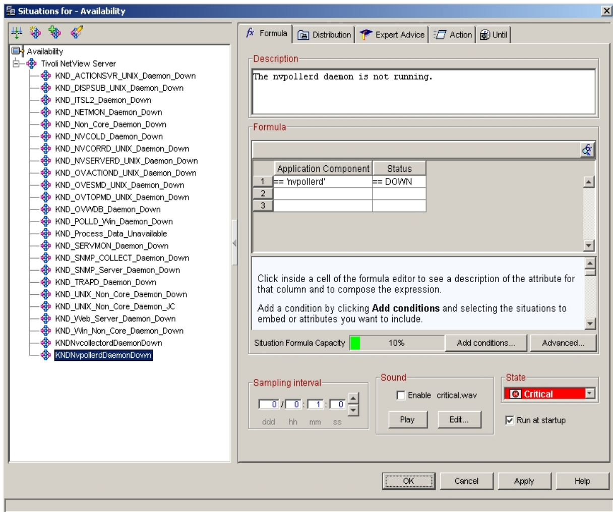
Figure 21: User defined situation to detect nvpollerd down
