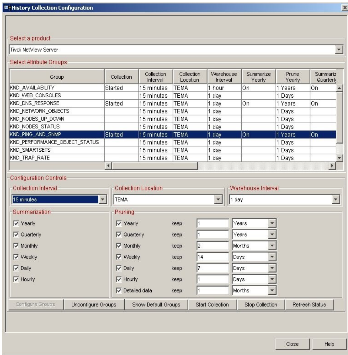
Figure 17: Configuring historical data collection for the NetView TEMA Attribute Groups
